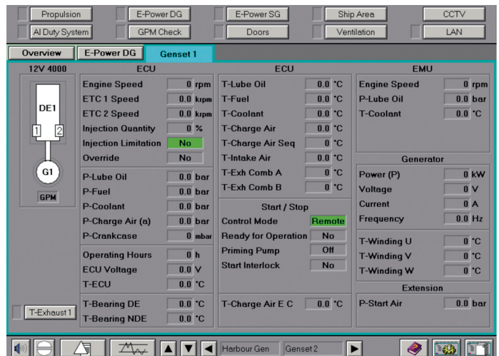
Visualization example: genset
